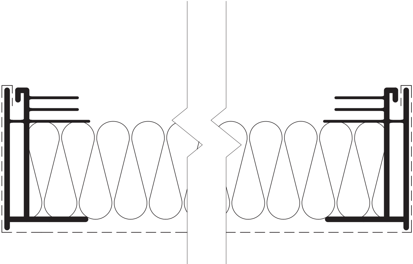
AcoustiCloud: 1-3/4" - Perimeter - Square Drawing Number: 13.1.00
