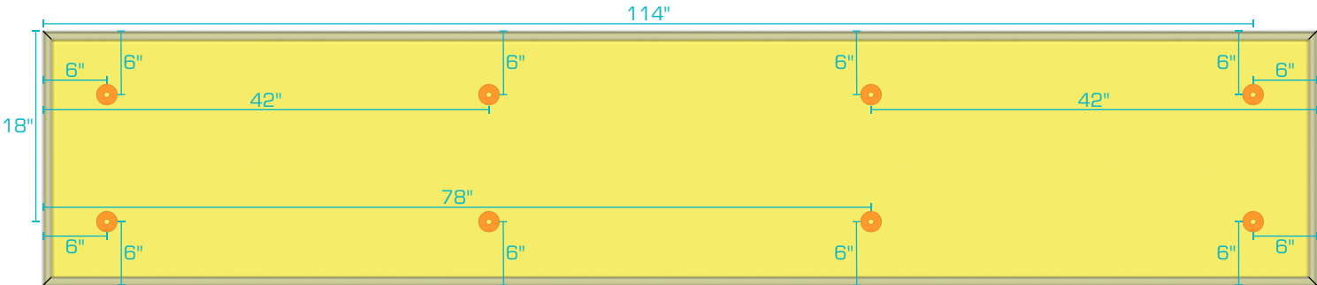
2' x 10' Panel
