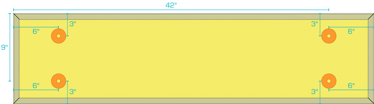
1' x 4' Panel
