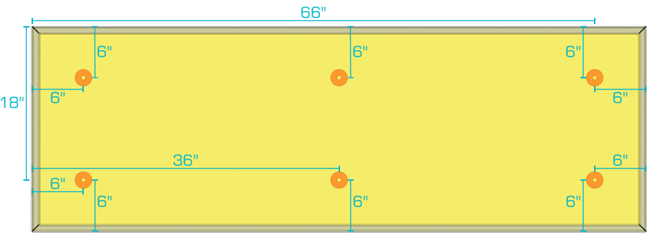
2' x 6' Panel
