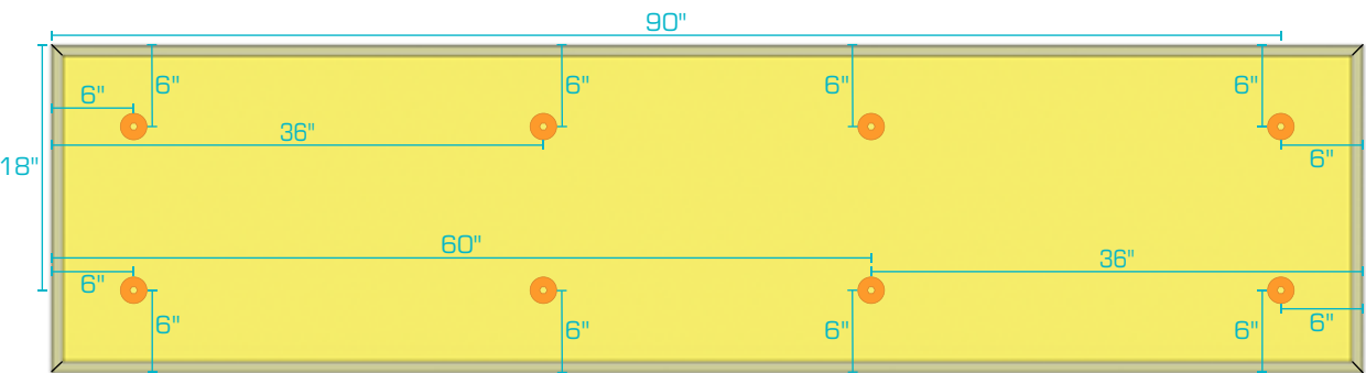
2' x 8' Panel
