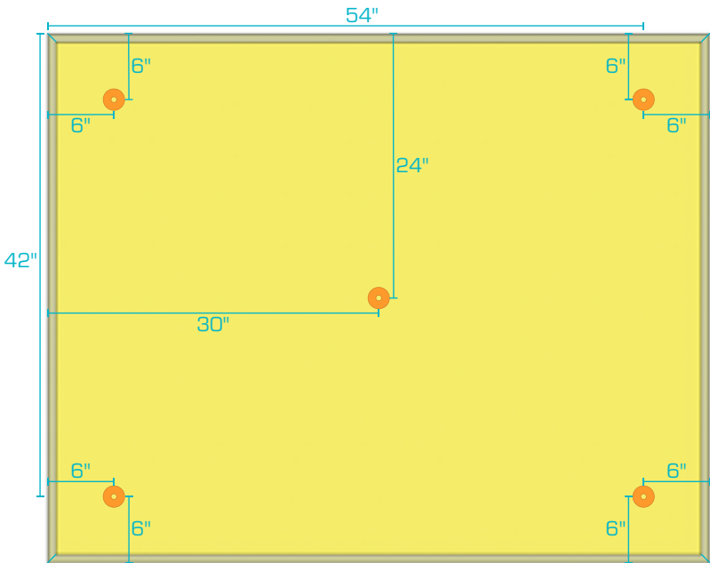
4' x 5' Panel
