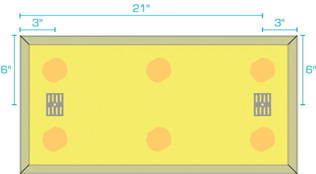
2' x 1' Panel
