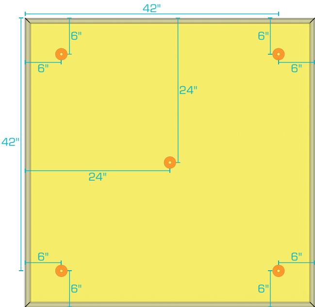
4' x 4' Panel
