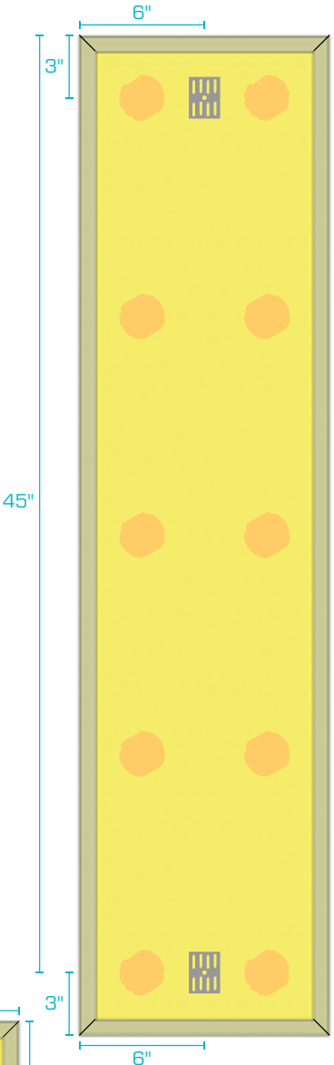
1' x 4' Panel
