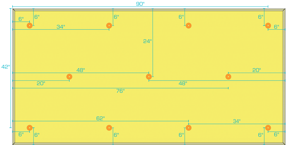
4' x 8' Panel
