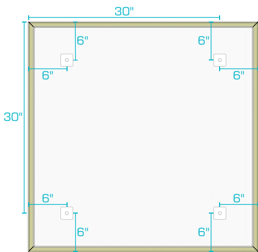
3' x 3' Panel
