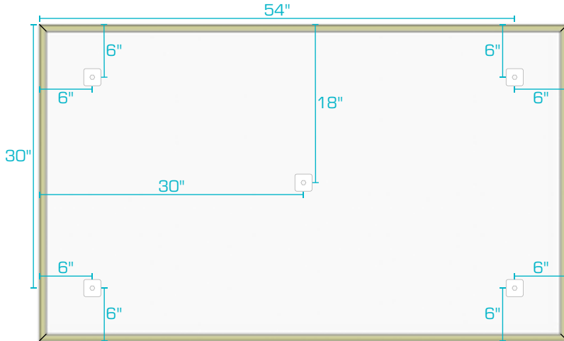
3' x 5' Panel
