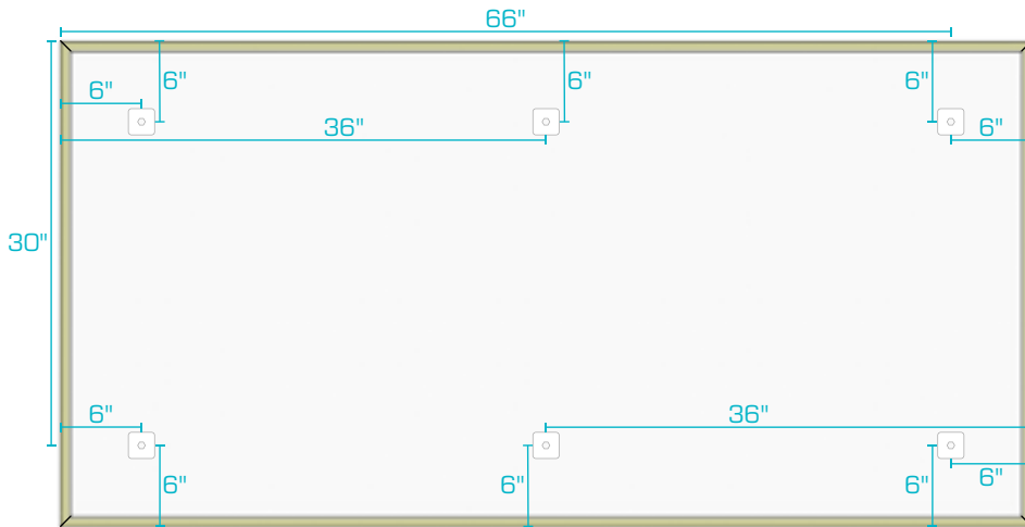
3' x 6' Panel
