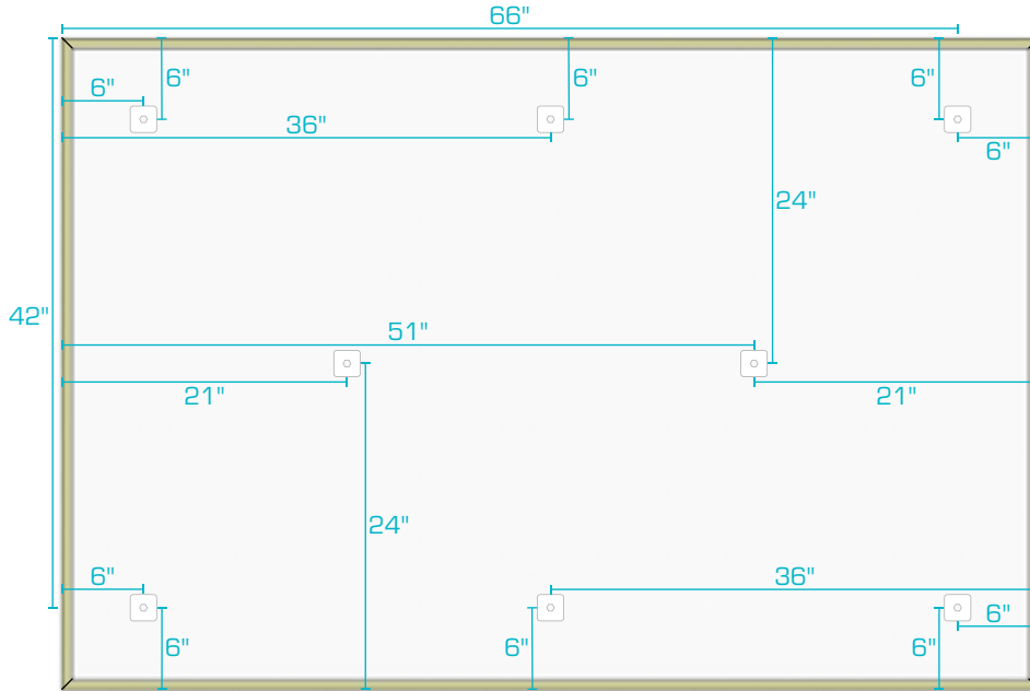
4' x 6' Panel
