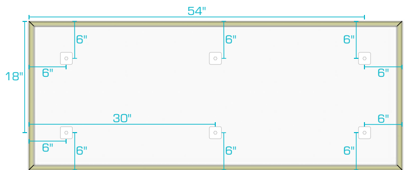
2' x 5' Panel
