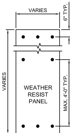
C L-11 ALTERNATE - WASHER PLATE DETAIL SCALE: NA
