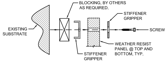
B L-11 HARDWARE ATTACHMENT DETAIL SCALE: NA
