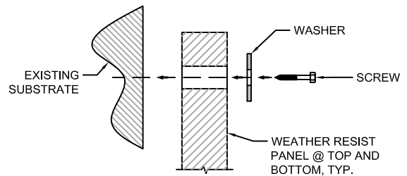
D L-11 ALTERNATE - HARDWARE ATTACHMENT DETAIL SCALE: NA
