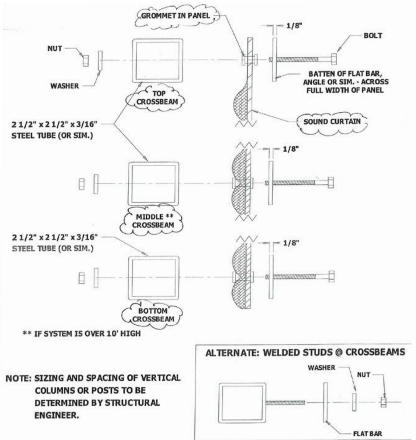
DETAIL: ATTACHMENT OF SOUND CURTAIN TO HORIZONTAL STRUCTURAL STEEL SUPPORTS
