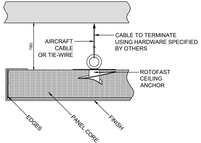
2 D-01 ROTOFAST CLOUD MOUNT ATTACHMENT SCALE: NA
